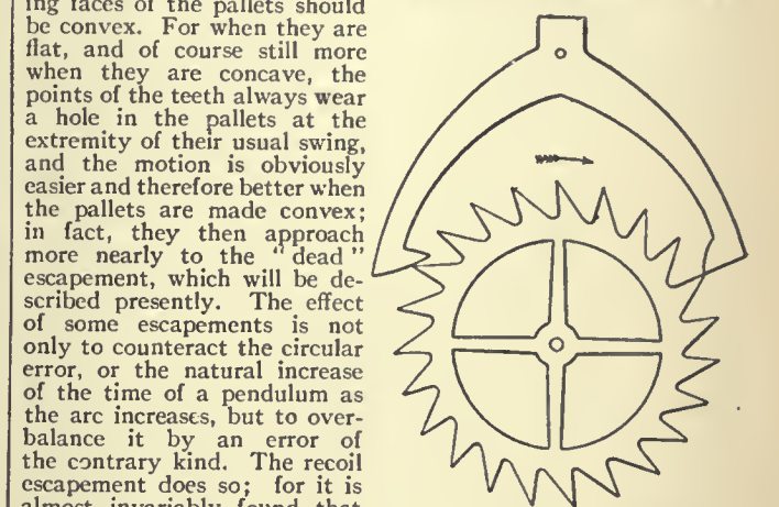
FIG. 8.—Anchor or Recoil Escapement.
